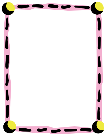
The Universe – BEFORE the Big Bang
