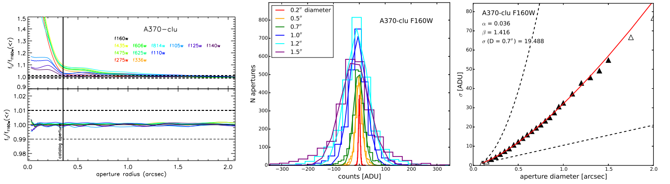
Figure A27. Same as Figures 8 and 9 but for the A370 cluster.
