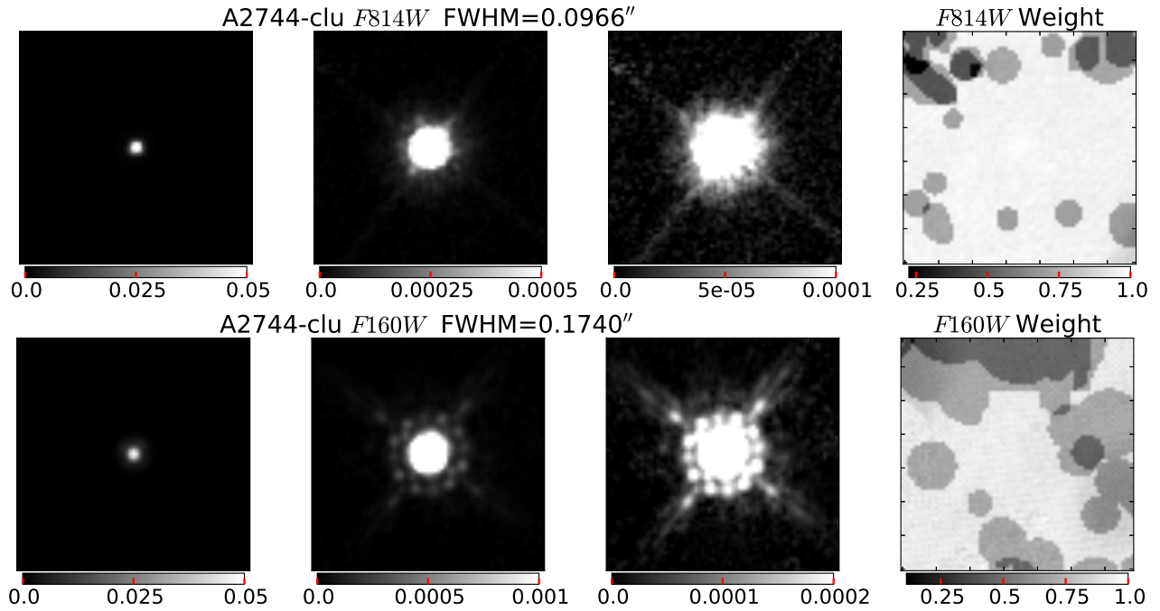
Figure A12. Same as Figure 6 but for the A2744 cluster. Point-spread functions (PSFs) for the ACS/ F814W band the WFC3/ F160W band. The construction of the PSFs is described in Section 3.4. For each filter we show three scales (top panels for F814W and bottom for F160W as labeled) to illustrate the structure of the PSF (from left to right : the core, the first Airy ring and the diffraction spikes). The images are normalized to a maximum value of one. The grayscale bars show the scale for each panel. These are different for the ACS and WFC3 as a result of the different FWHMs (listed above the images). We also show the combined weight images for each PSF. The weight is largest in the center and lower at larger radii and not consistent as shown due to masking of neighboring objects (this is the reason for darker circles appearing).
