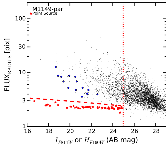
Figure A42. Same as Figure 10 but for the M1149 parallel.
